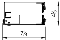
TRACK DETAIL 3:1
